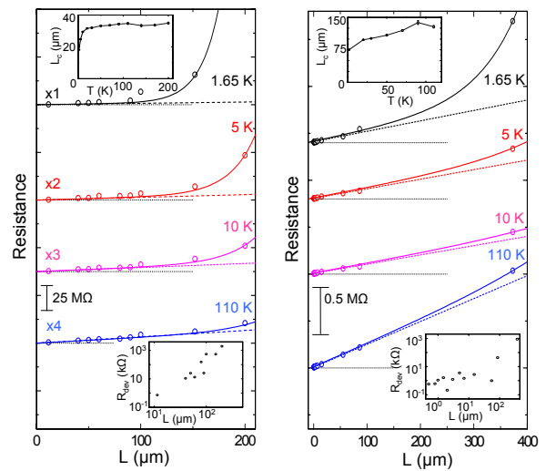
FIG. 4: R(L) in the non-linear regimes for samples (a) SC6 ( L_m^{\text{sat}} \approx 460 \text{ nm} ) and (b) M3 ( L_m^{\text{sat}} \approx 7 \mu\text{m} ). Note that the data is magnified in (a) for clarity. The dashed line is an extension of the linear regime and the solid line is a fit for all data. R_{\text{dev}} shows the absolute value of the difference between the actual device resistance and the corresponding linear resistance at 110 K (lower inset a) and 1.65 K (lower inset b). The non-linearity increases with decreasing temperature, which is reflected in the value of L_c (upper insets).
